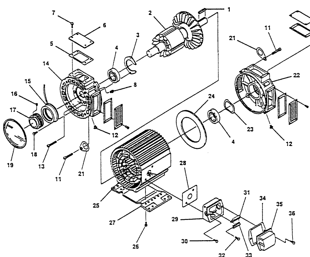
PACTORQ "E" Series Brushless DC Motor Exploded View and Parts List
